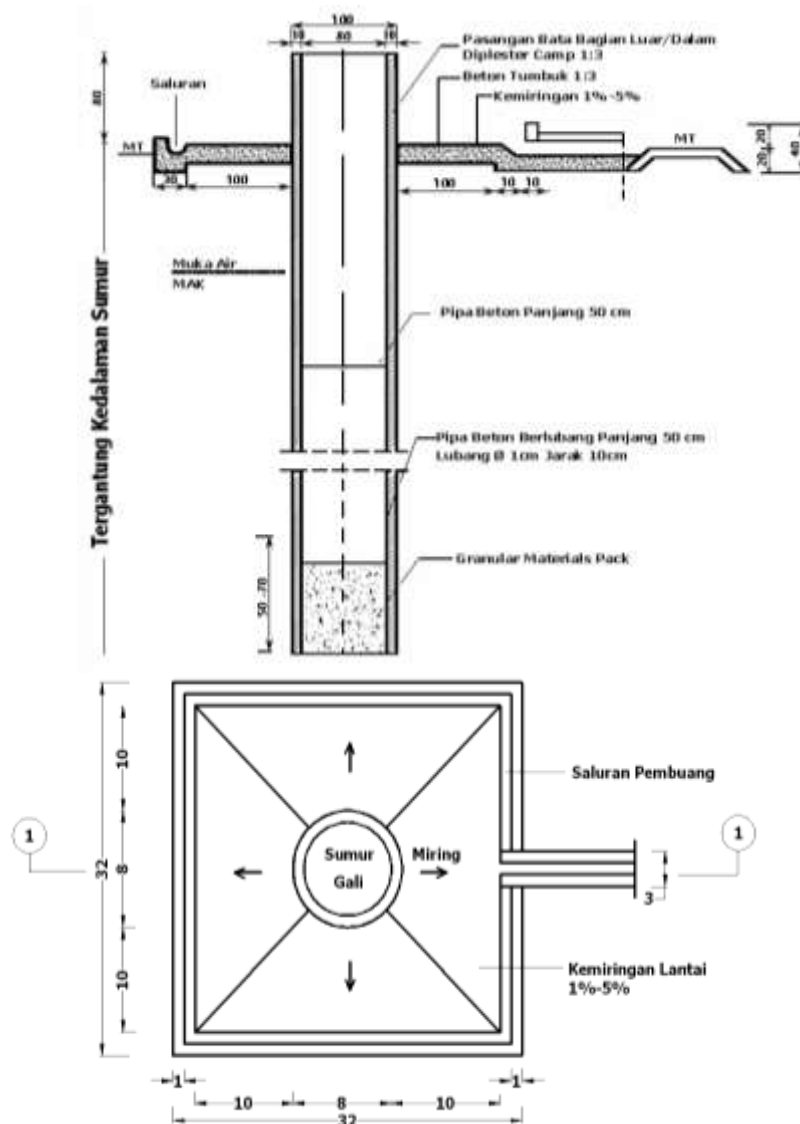
Gambar 3.17 Model Sumur Gali/Sumur Dangkal
